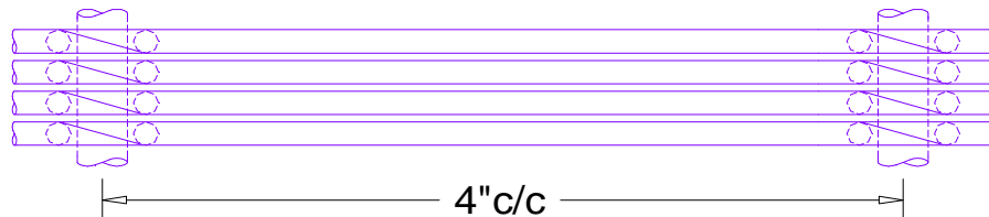
Plan View A-A (Screen Detail 20x)
